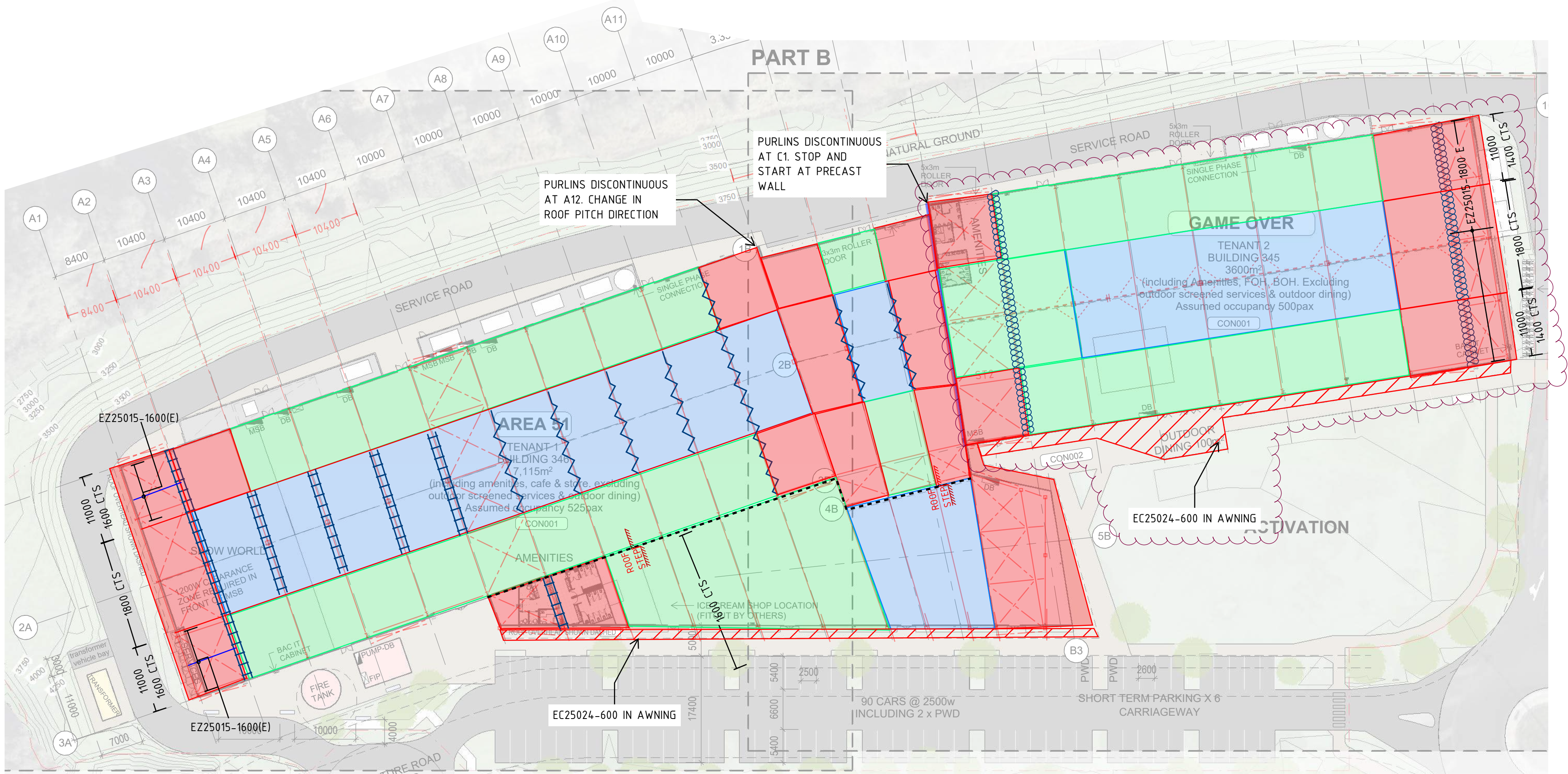
PURLIN PLAN
